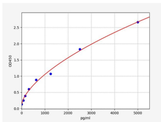
Standard curve for orb563283 ELISA kit.
