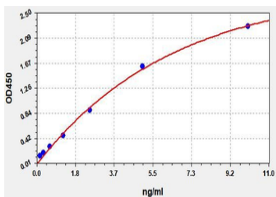
Standard curve for orb562981 ELISA kit.
