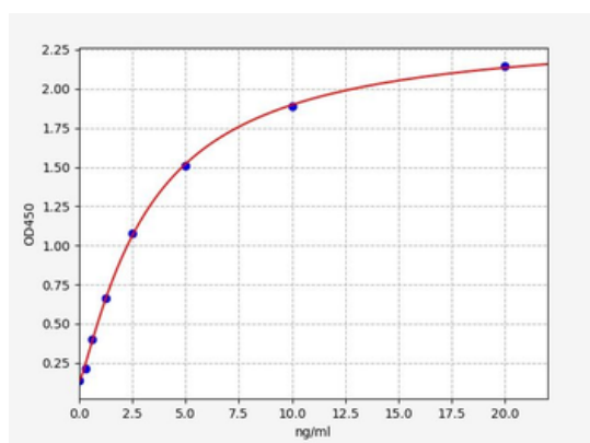
Standard curve for orb562886 ELISA kit.
