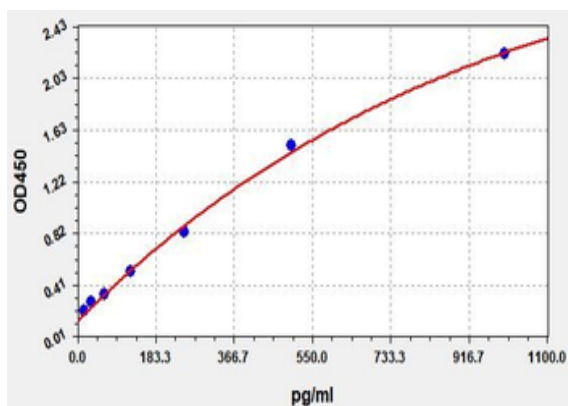
Standard curve for orb562365 ELISA kit.
