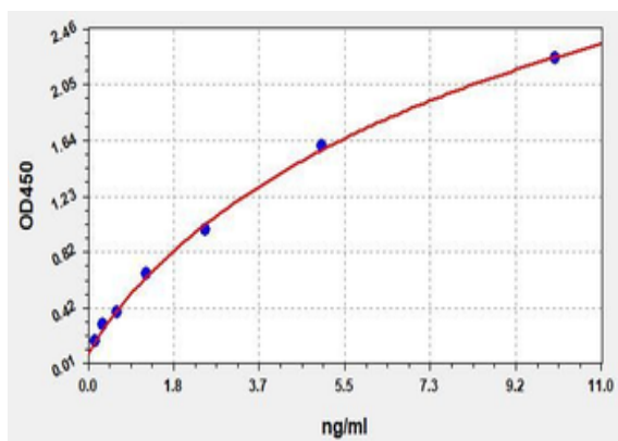
Standard curve for orb561900 ELISA kit.
