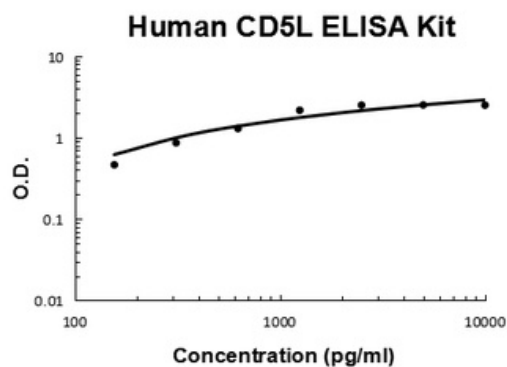
Human CD5L PicoKine ELISA Kit standard curve
