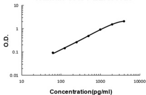
Human GAS6 PicoKine ELISA Kit Standard Curve
