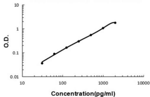
Human TREM-1 PicoKine ELISA Kit Standard Curve
