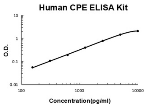
Human CPE PicoKine ELISA Kit standard curve
