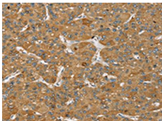
Immunohistochemistry of paraffin-embedded Human liver cancer tissue using SENP3 antibody
