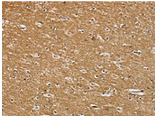
Immunohistochemistry of paraffin-embedded Human brain tissue using SENP3 antibody
