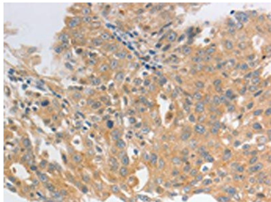
Immunohistochemistry of paraffin-embedded Human ovarian cancer tissue using HCRTR2 antibody
