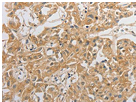
Immunohistochemistry of paraffin-embedded Human lung cancer tissue using HCRTR2 antibody
