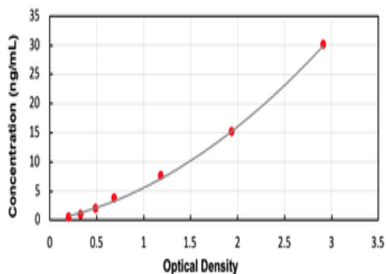
Standard curve for orb440475 ELISA kit.
