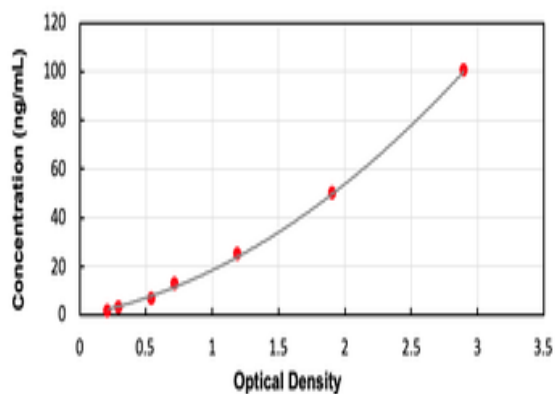
Standard curve for orb439511 ELISA kit.
