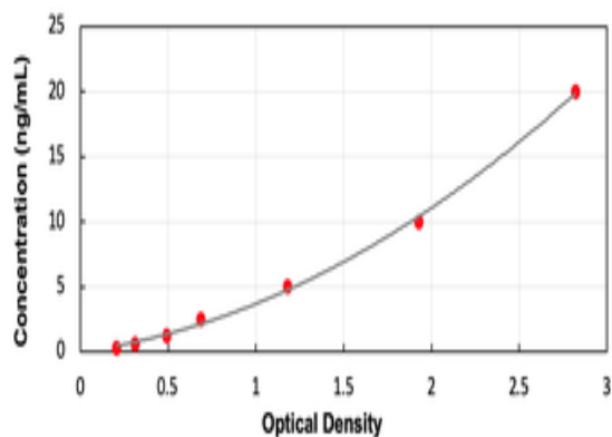
Standard curve for orb439294 ELISA kit.
