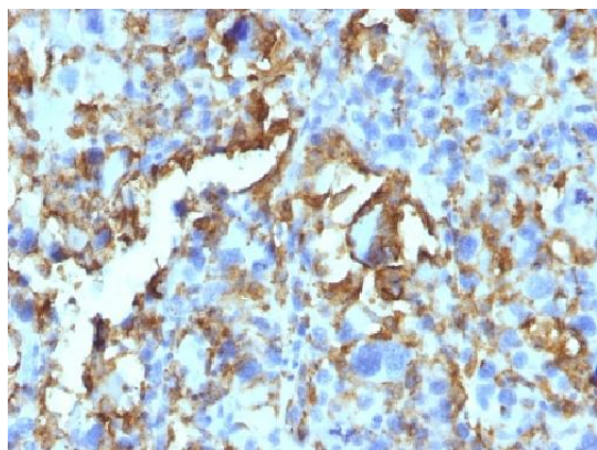
Immunohistochemical staining of human Histiocytoma tissue using HLA-DRB1 antibody
