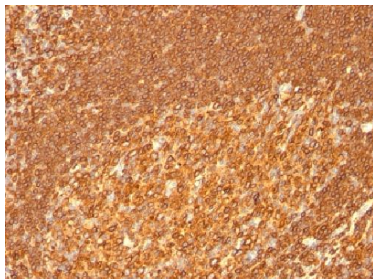
Immunohistochemical staining of human Tonsil tissue using HLA-DRB1 antibody
