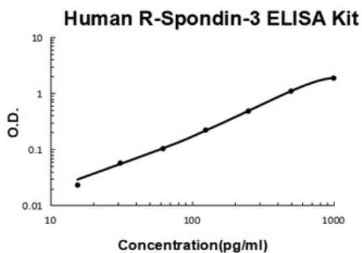
Human R-Spondin-3 PicoKine ELISA Kit standard curve
