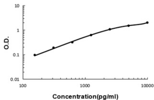
Mouse EPCR PicoKine ELISA Kit standard curve
