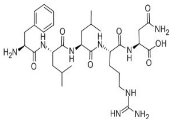
Chemical structure of orb372881.
