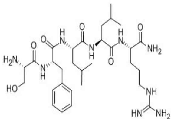
Chemical structure of orb372880.
