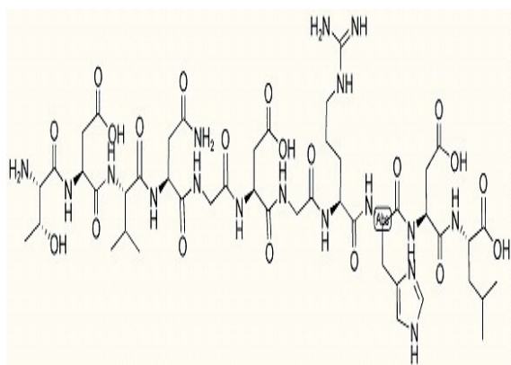
Chemical structure of orb372716.
