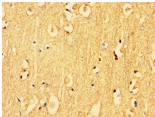
Immunohistochemical staining of human brain tissue using KLK6 antibody
