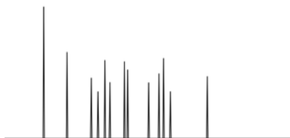
Taxane Standard Mixture
