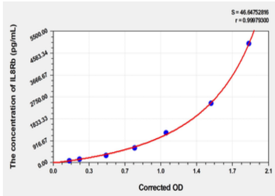
Standard curve for orb2999536 ELISA kit.
