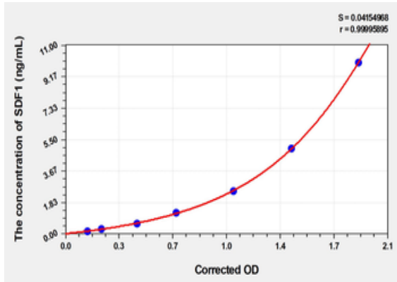
Standard curve for orb2999086 ELISA kit.
