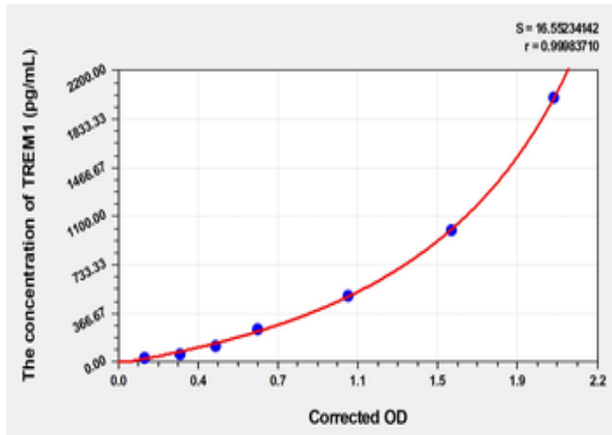
Standard curve for orb2999058 ELISA kit.
