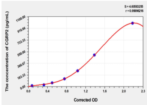
Standard curve for orb2999025 ELISA kit.
