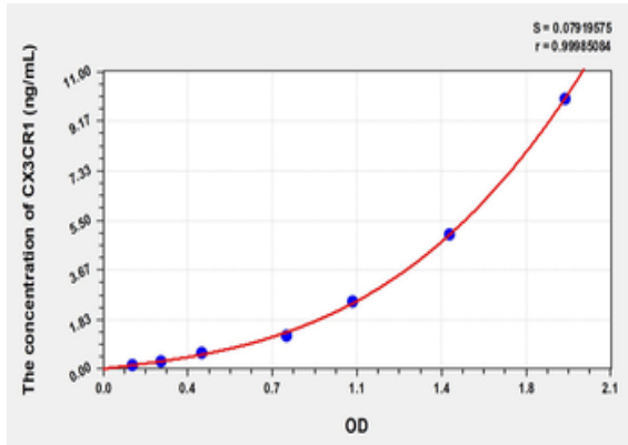
Standard curve for orb2998565 ELISA kit.
