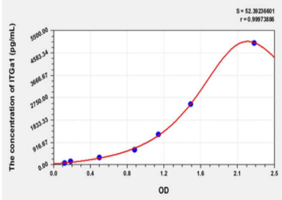
Standard curve for orb2998350 ELISA kit.
