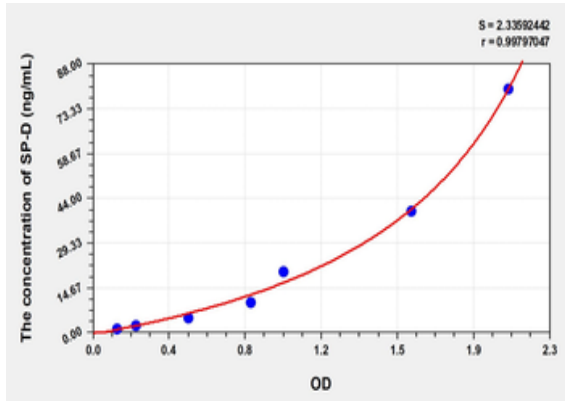
Standard curve for orb2997470 ELISA kit.
