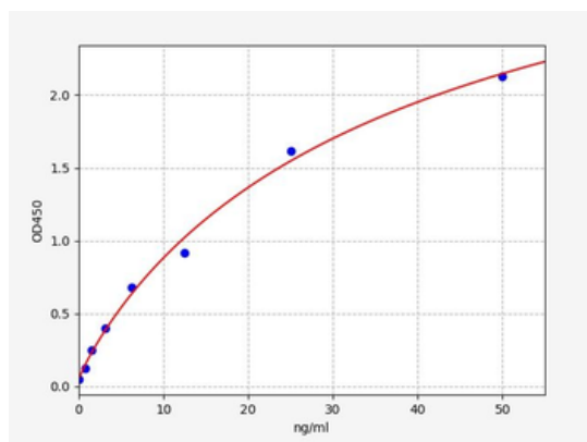
Standard curve for orb2938798 ELISA kit.
