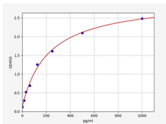
Standard curve for orb2647797 ELISA kit.
