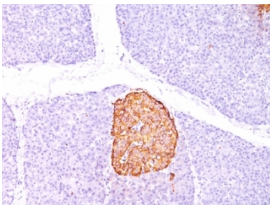
IHC: Formalin-paraffin human pancreas stained with Chromogranin A antibody (CHGA/798)
