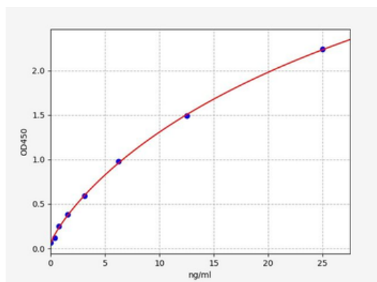
Standard curve for orb2567673 ELISA kit.
