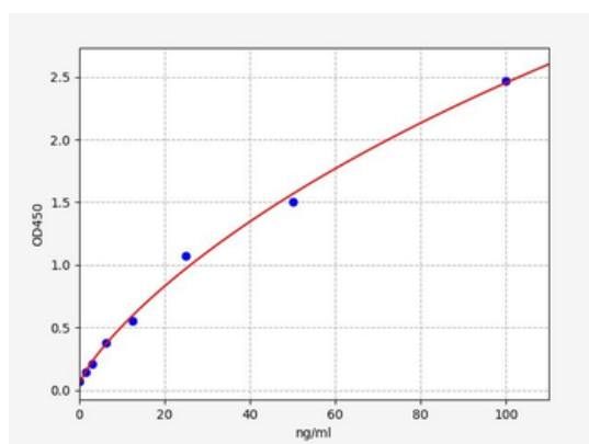
Standard curve for orb2567545 ELISA kit.
