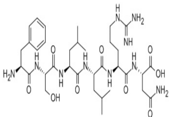
Chemical structure of orb233780.
