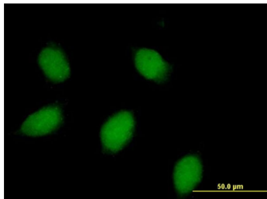
Immunofluorescence of purified MaxPab rabbit antibody to CALB1 on HeLa cell. [antibody concentration 10 ug/ml].
