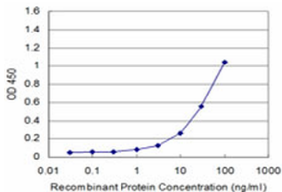
Detection limit for recombinant GST tagged CDK4 is approximately 3 ng/ml as a capture antibody.
