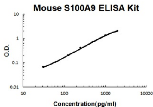
Mouse S100A9 PicoKine ELISA Kit standard curve
