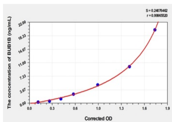
Standard curve for orb1736598 ELISA kit.
