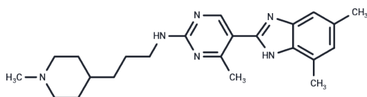
Chemical structure of toreforant
