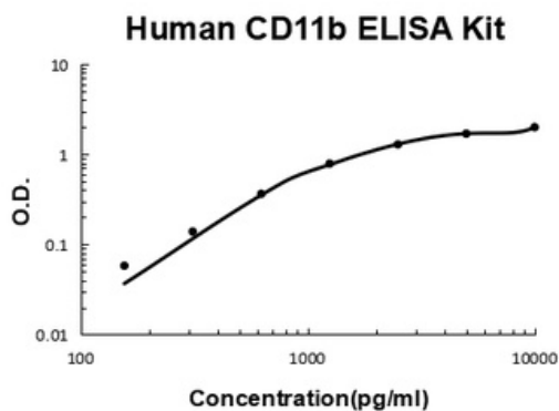
Human CD11b PicoKine ELISA Kit standard curve
