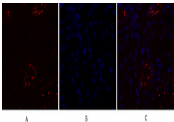
IF analysis of orb1412845.
