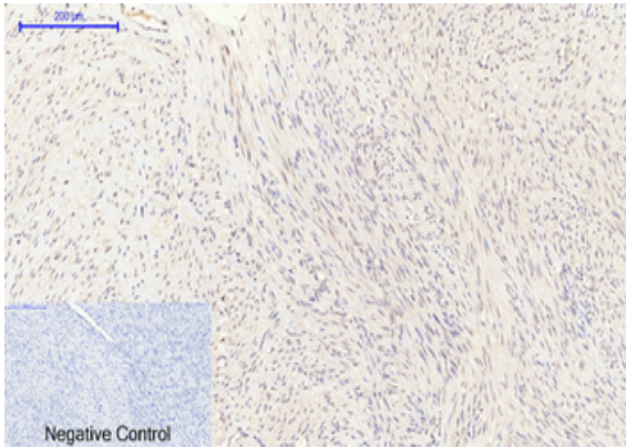
IHC analysis of orb1412845.
