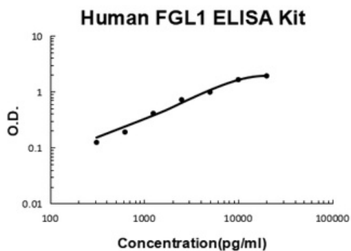
Human FGL1 PicoKine ELISA Kit standard curve
