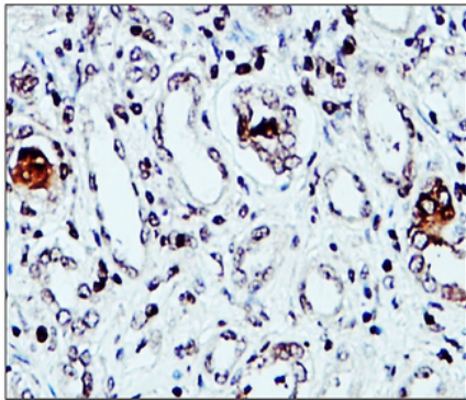
Kidney carcinoma
