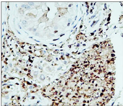
Liver carcinoma
