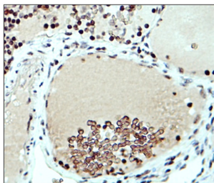
Breast carcinoma
