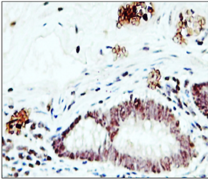
Colorectal carcinoma
