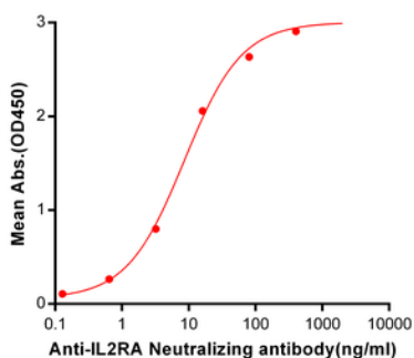
Anti-IL2RA (basiliximab biosimilar) mAb ELISA 0.2 µg of Human IL2RA, His Tagged protein per well
