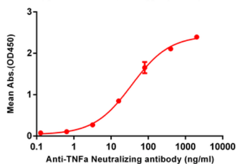
Anti-TNF \alpha (Adalimumab biosimilar) mAb ELISA 0.1 \mu g of Human TNF \alpha , His Tagged protein per well
