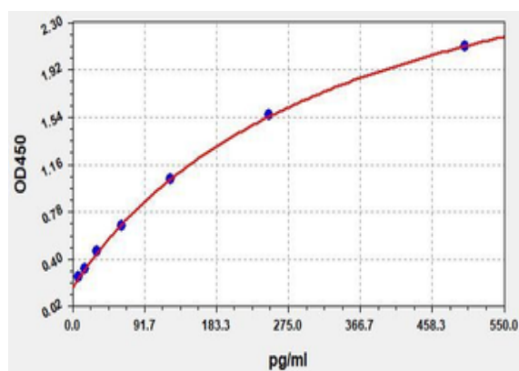
Standard curve for orb1101093 ELISA kit.
