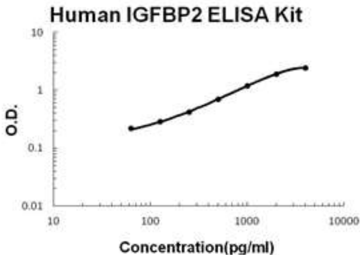
Human IGFBP2 PicoKine ELISA Kit standard curve
