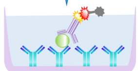
Stop solution
