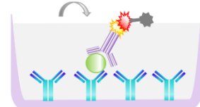
Streptavidin-HRP
