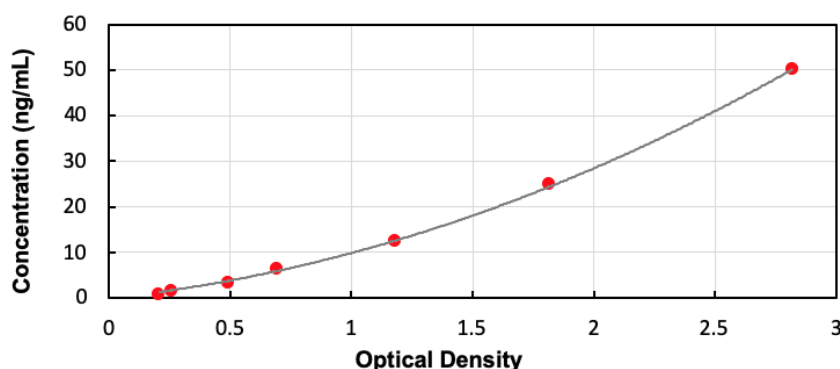
Typical Standard Curve for Human SOD2 ELISA
